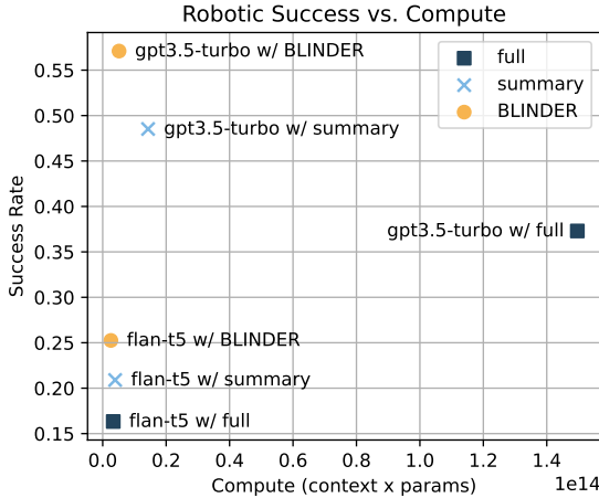
Figure 6: Success rates on our robotic object arrangement task when using BLINDER vs. base-lines for state descriptions. The actor is tasked with arranging two, three, or four items. The GPT3.5 Turbo Actor once again outperforms the T5 actor, and BLINDER continues to generalize well despite being trained with the T5 actor.
